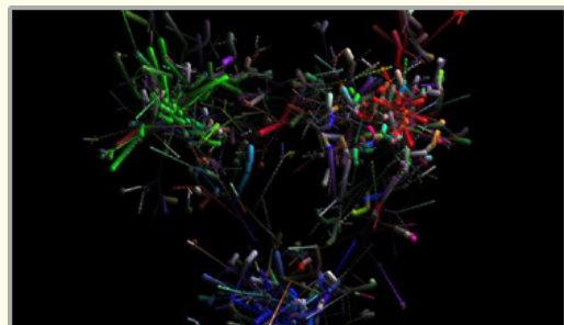
Figure 3: Physical Vacuum fluctuation.
