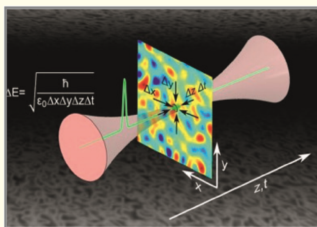
Figure 4: Physical Vacuum polarization.
